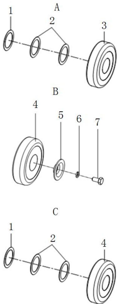
Fig. I Cross roller assy
