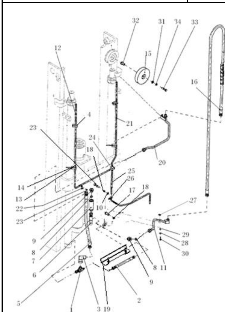
Fig.28 Mast piping
