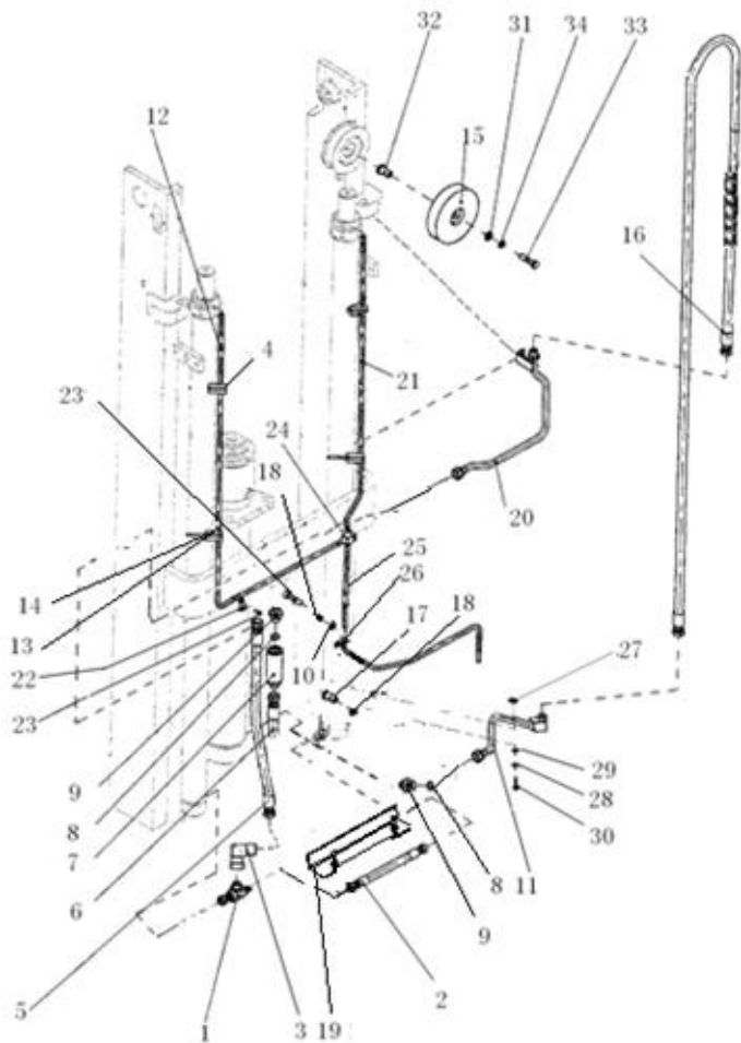
Fig.28 Mast piping
