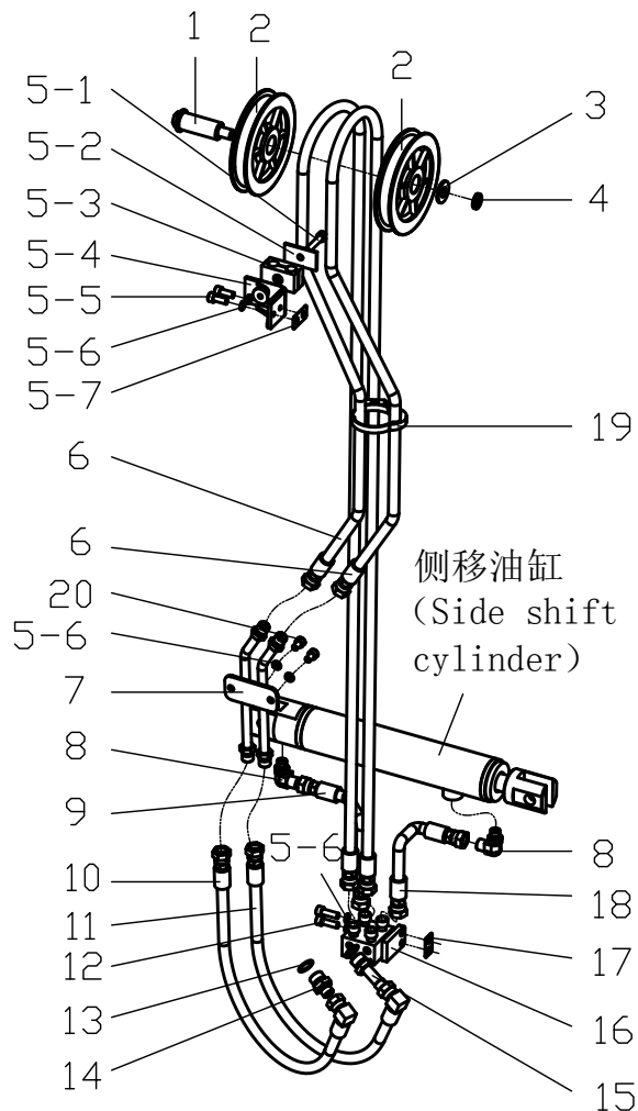
Fig.10 lateral moving circuit
