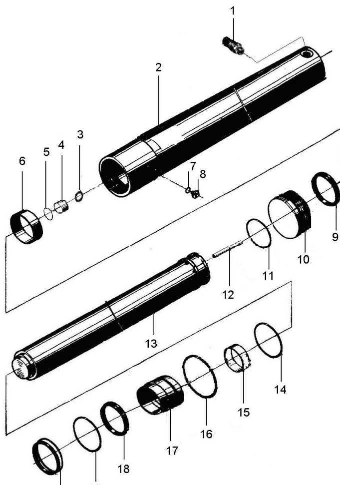
图 27 短升降油缸 Fig.27 Lift cylinder, Short
